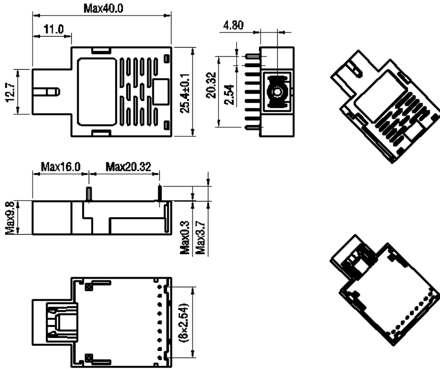
SC receptacle middle output
