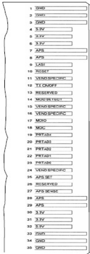
Top view -Top side of PCB
