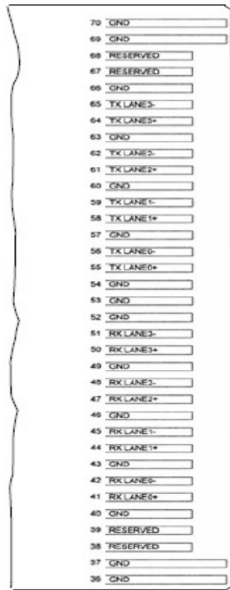
Top view-Bottom side of PCB
