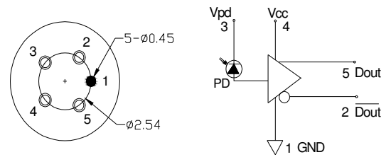
PIN-TIA-pin-D
